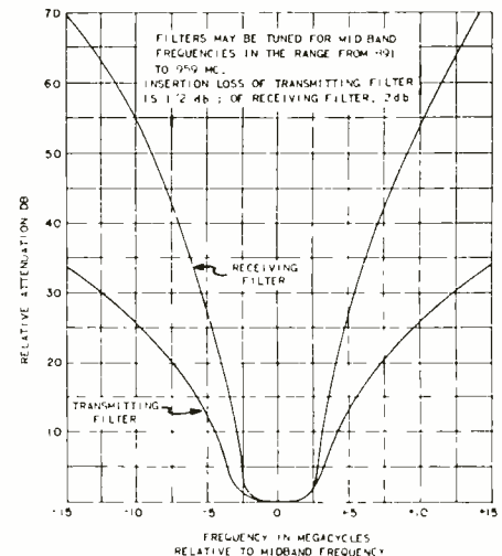
Fig. 3. Curves showing the frequency response of transmitting and receiving filters. Two series cavities are used for transmitting and four for receiving.
