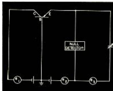
Fig. 6. Modified \mu bridge circuit for measuring the h_{12} characteristic of junction transistors.
