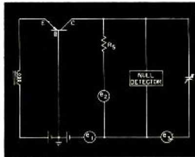
Fig. 4. Modified R_p bridge circuit designed to measure the h_{22} characteristic of junction transistors.
