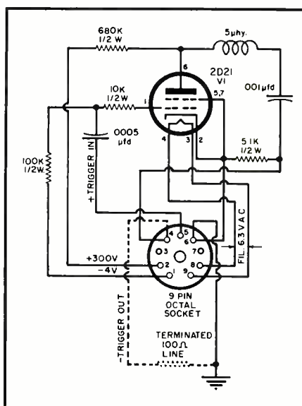
Fig. 6. Schematic diagram and parts values for thyatron pulse shaper.
