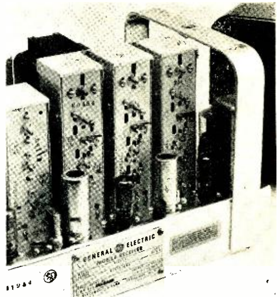
Fig. 1. In converting from wide-band to narrow-band operation, the first step is to remove the three low i.f. transformers from the receiver chassis.
