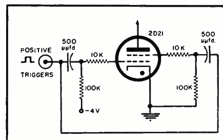
Fig. 7. Triggering circuit in which both grids are pulsed simultaneously.
