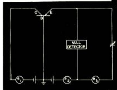
Fig. 2. Simplified bridge circuit for measuring R_p of a vacuum tube.
