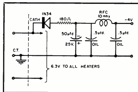
Fig. 5. Schematic diagram and parts values for a compact bias supply.
