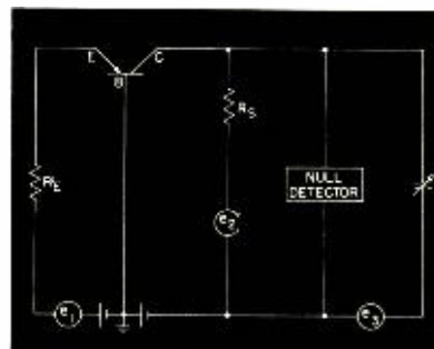
Fig. 8. Modified G_m bridge circuit for measuring the h_{21} characteristic of junction transistors.
