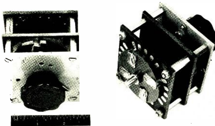
Fig. 6. Two views of a rotary switch with a printed circuit stator. This switch is manufactured for commercial applications by the Daven Company.
