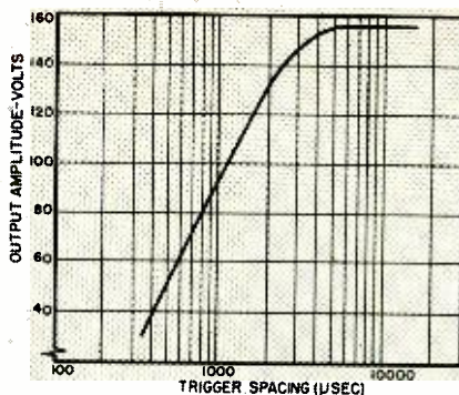
Fig. 2. Output amplitude vs. input trigger spacing for a fixed load and a 680\text{-}\mu\text{sec.} plate time constant.
