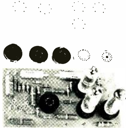
Fig. 4. Experimental five-tube a.c.-d.c. amplifier made with printed circuit technique, miniature tube socket adapters, and Auto-Semby system of fabrication.
