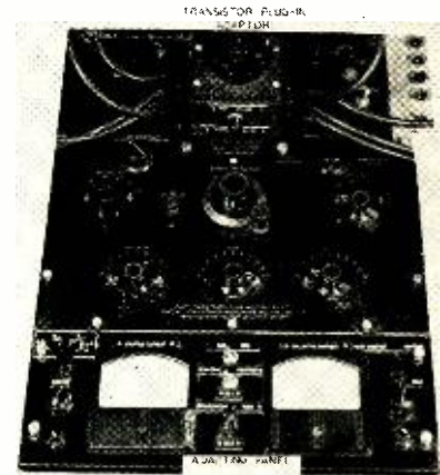
General Radio vacuum tube bridge Type 561-D adapted for transistor measurements.
