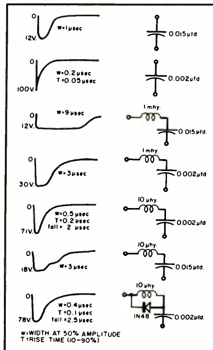
Fig. 4. Output waveshapes and plate circuit elements for basic unit.
